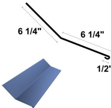
TF TRANSITION
