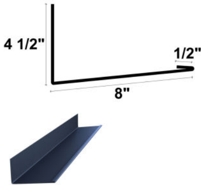
CHIMF CHIMNEY
