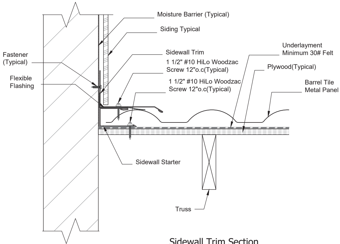
Sidewall Trim Section Scale 3"=1'
