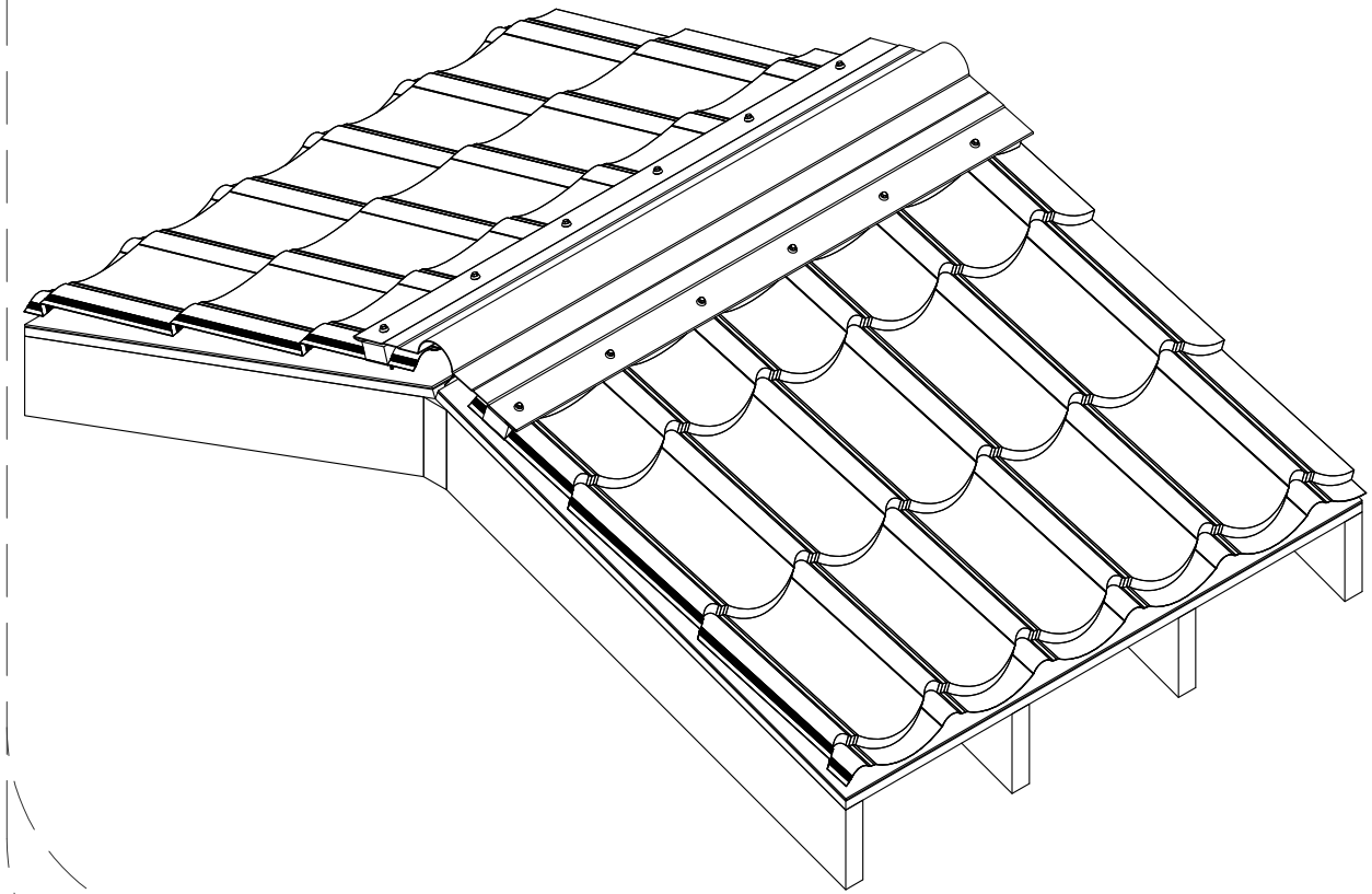
Isometric View
