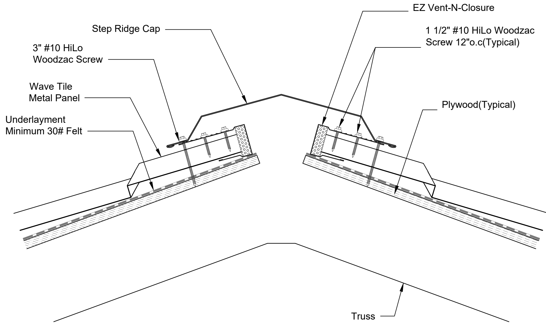
Roof Ridge Section Scale 3"=1'
