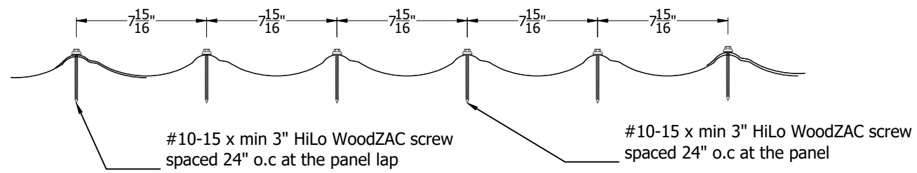
Fastening Pattern For Non-HVHZ Construction
