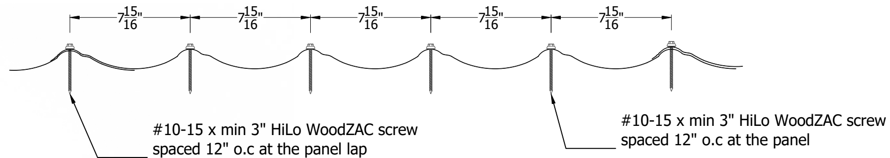
Fastening Pattern For HVHZ Construction
