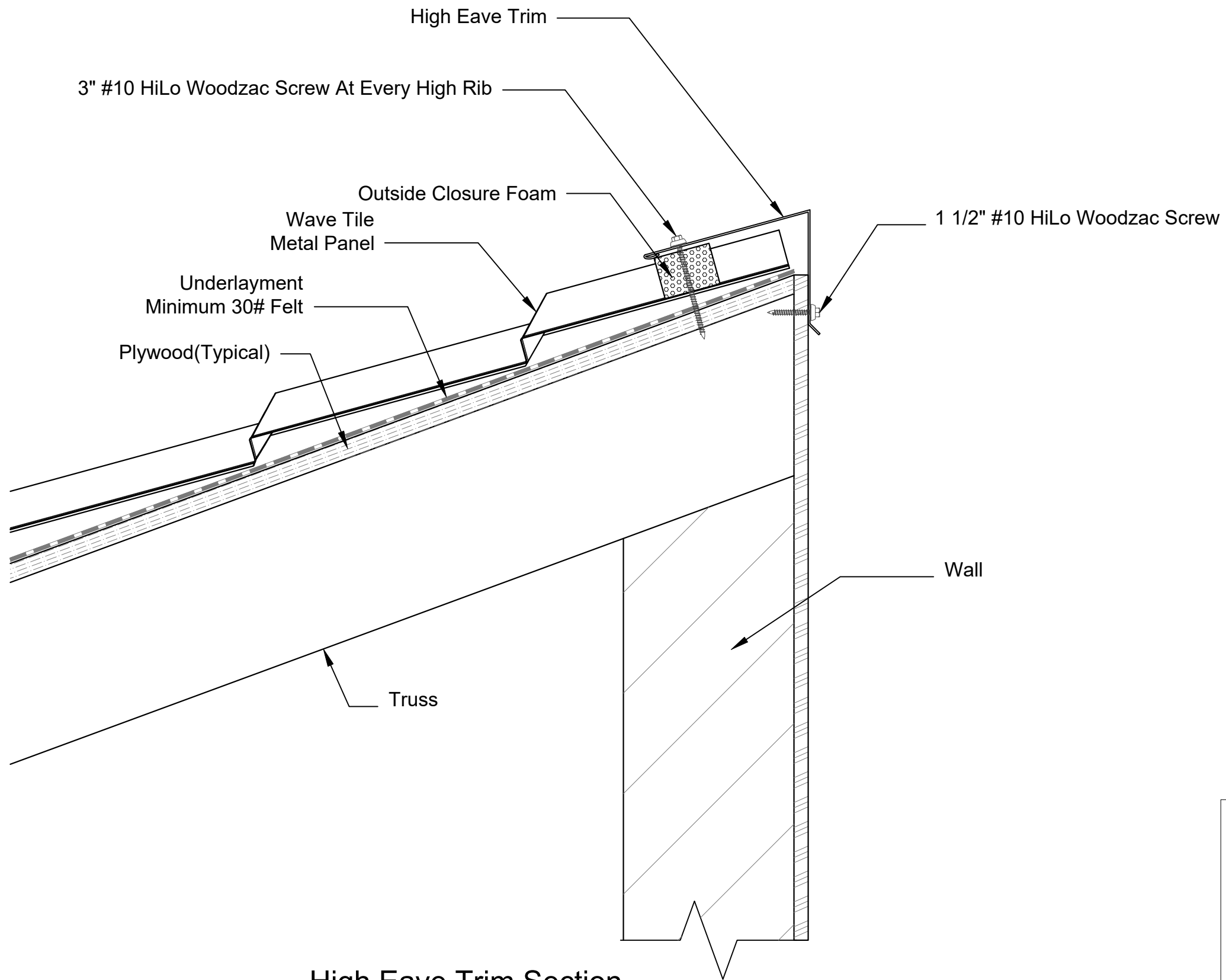
High Eave Trim Section Scale 3"=1'
