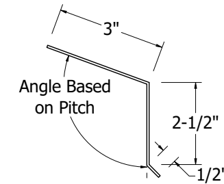
Standard Eave Drip Detail
