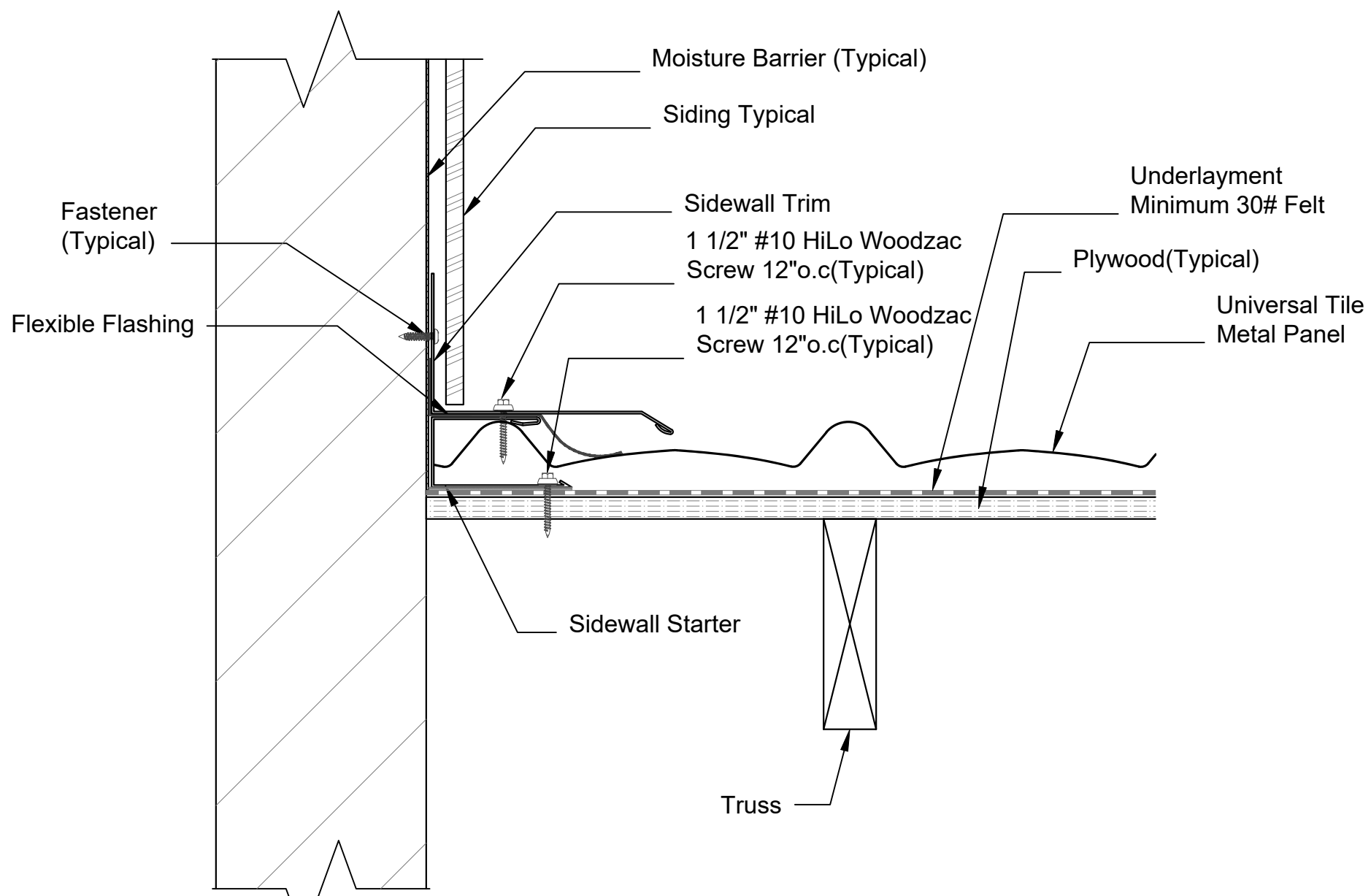
Sidewall Trim Section Scale 3"=1'
