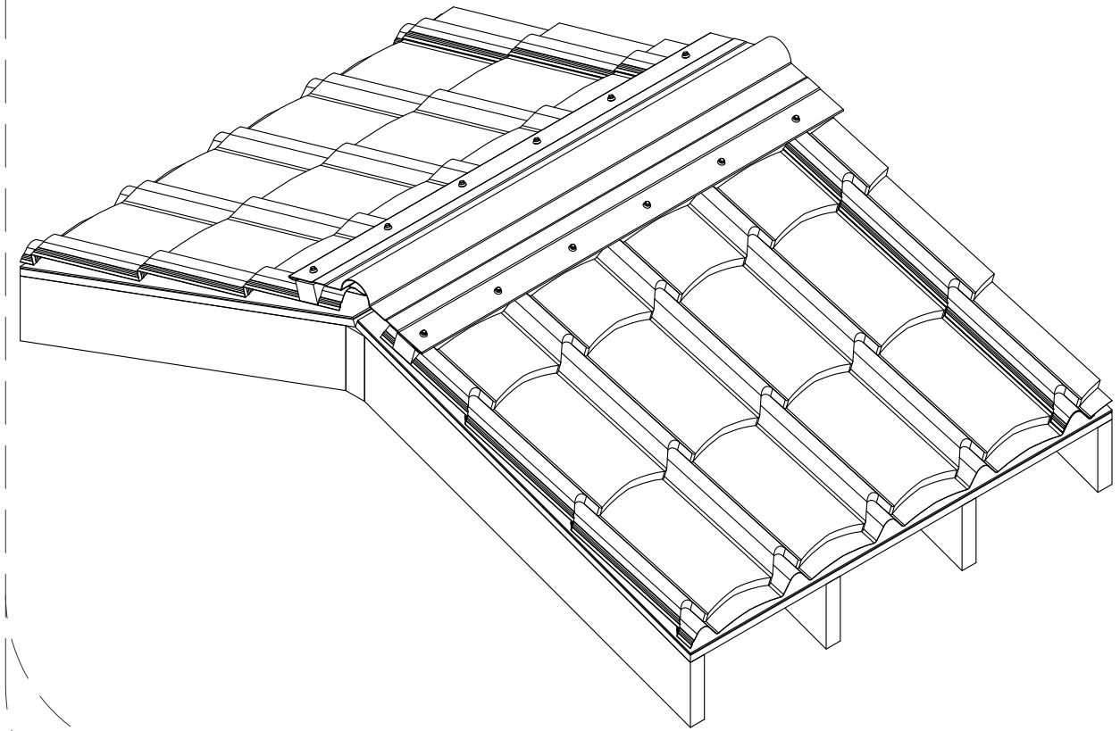
Isometric View
