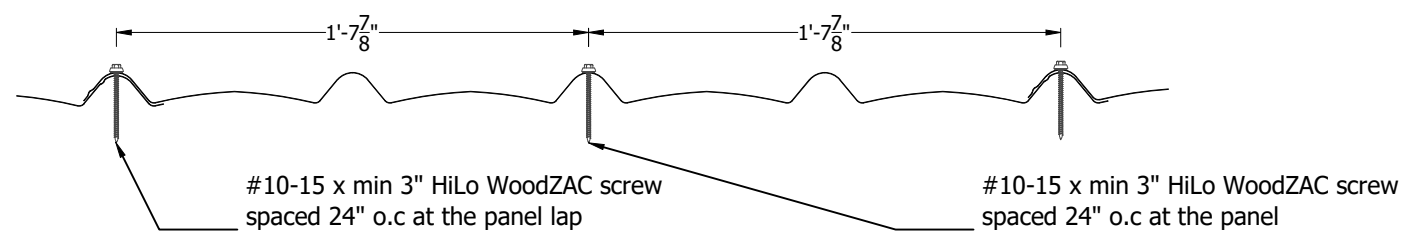
Fastening Pattern For Non-HVHZ Construction
