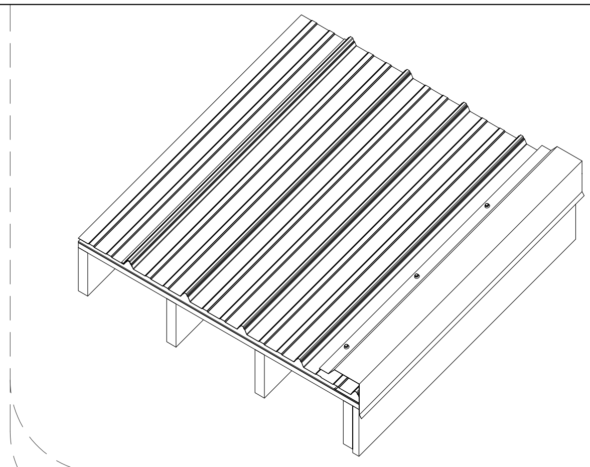
Isometric View
