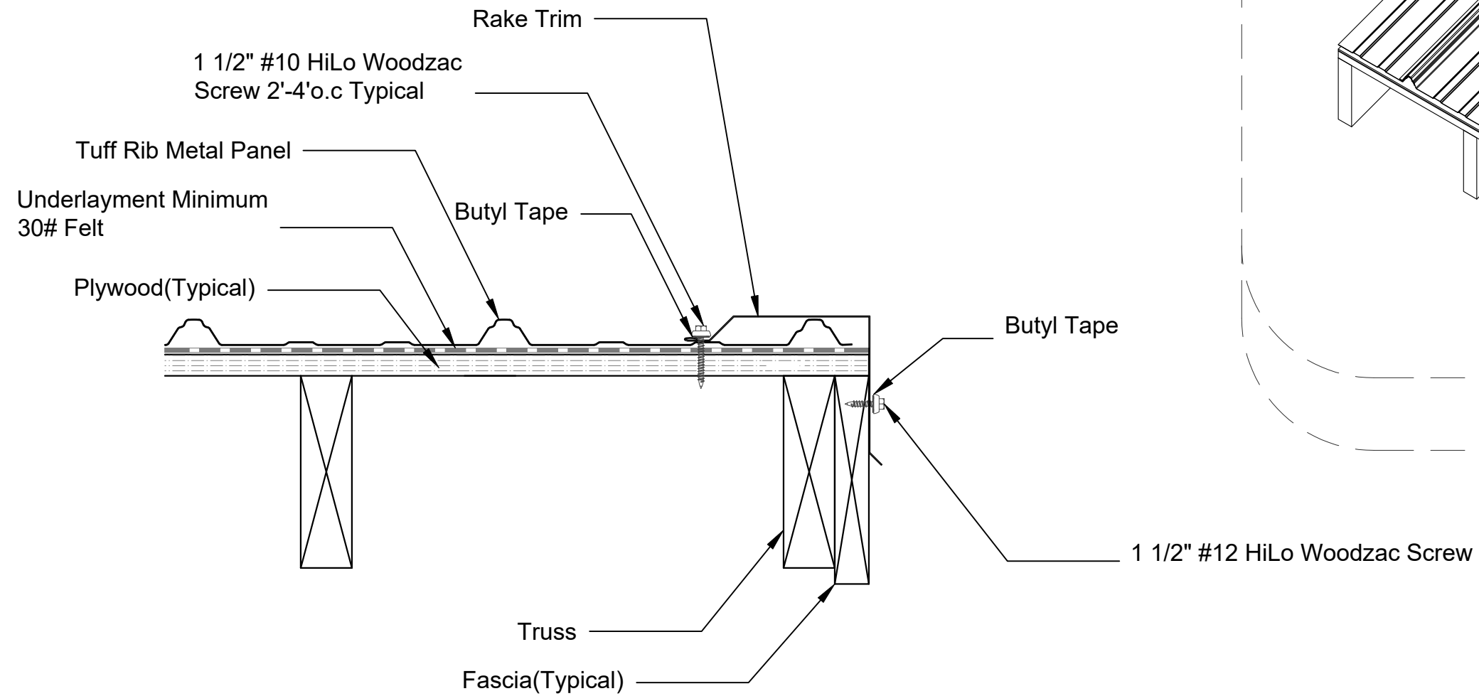
Rake Trim W/ Starter Section Scale 3"=1'
