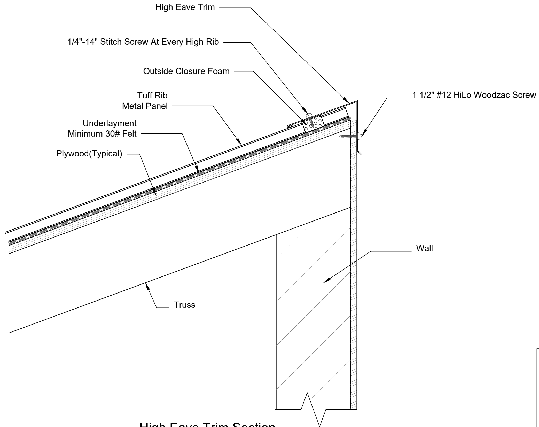
High Eave Trim Section Scale 3"=1'
