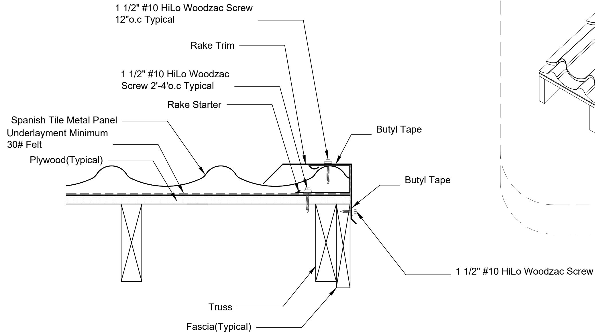
Rake Trim W/ Starter Section Scale 3"=1'
