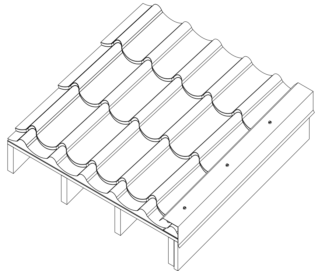
Isometric View
