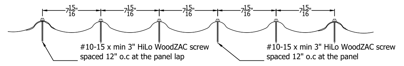
Fastening Pattern For HVHZ Construction
