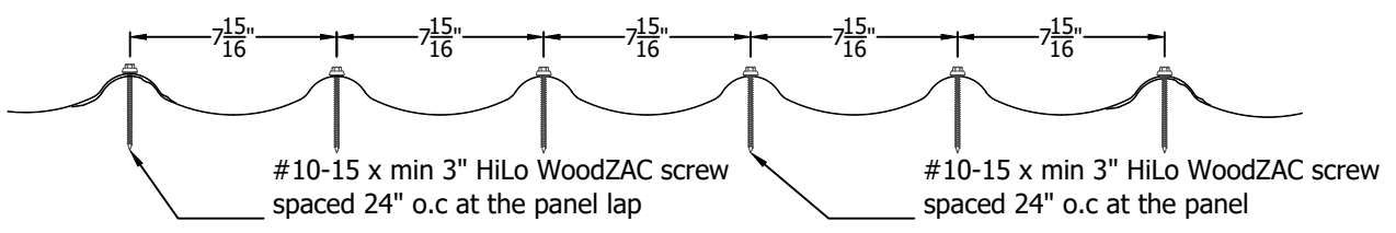
Fastening Pattern For Non-HVHZ Construction
