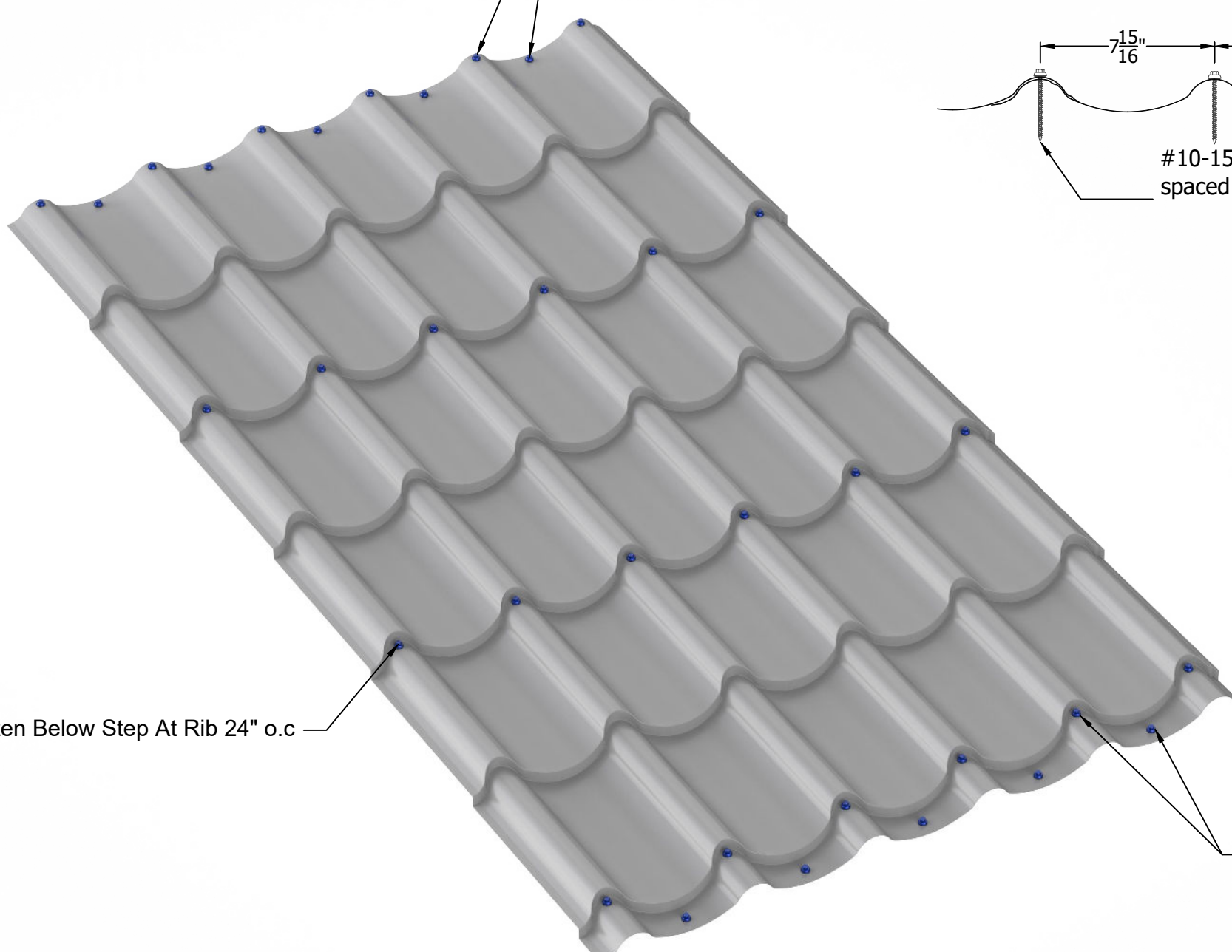
Fastening Pattern For Non-HVHZ Construction
