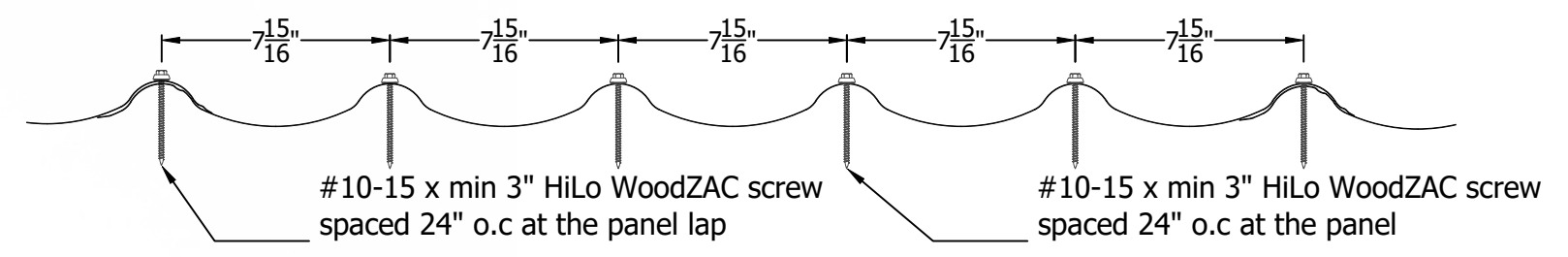
Fastening Pattern For Non-HVHZ Construction
