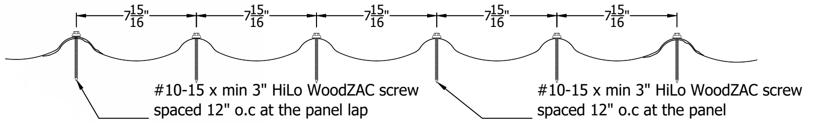
Fastening Pattern For HVHZ Construction
