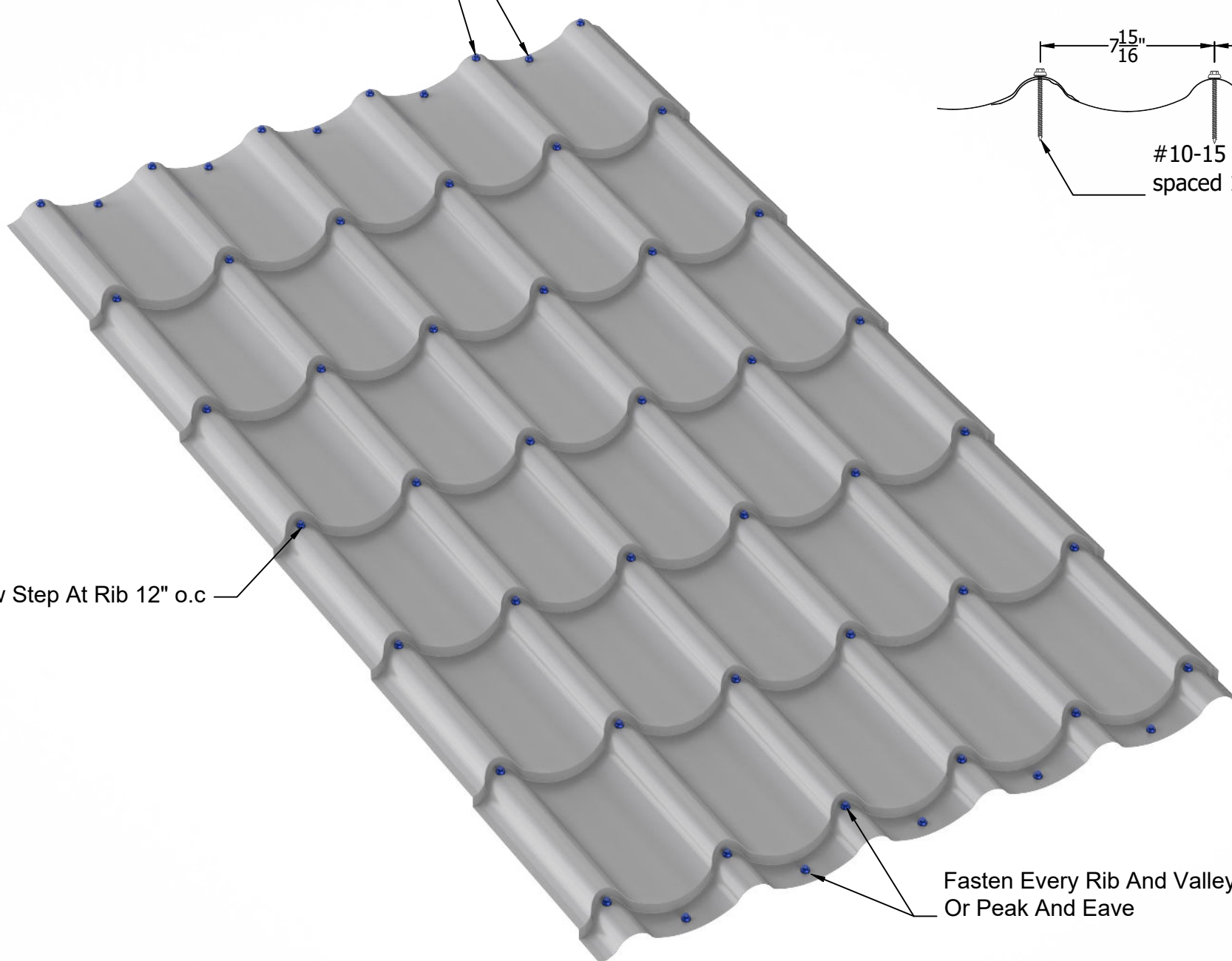
Fastening Pattern For HVHZ Construction
