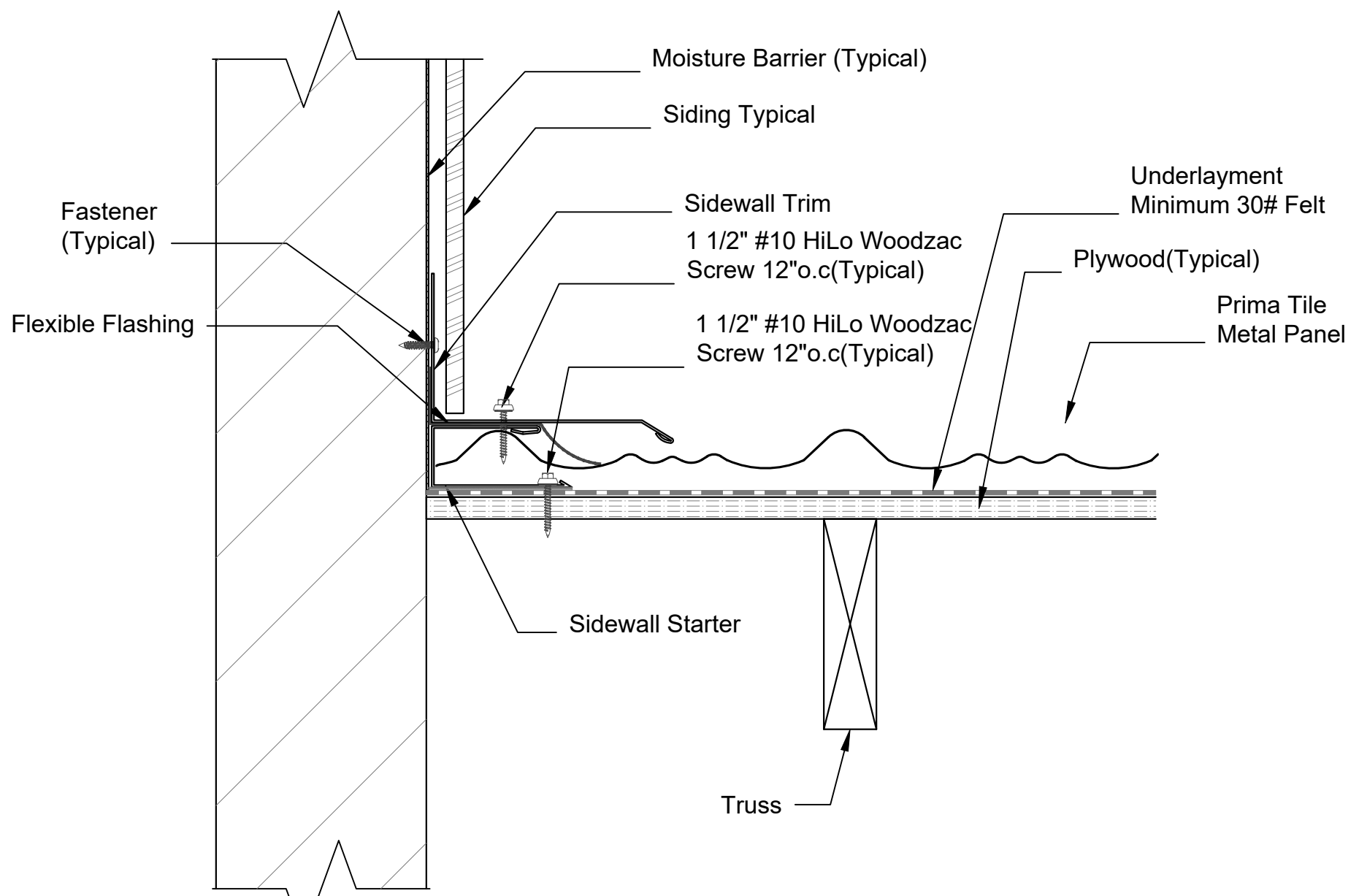
Sidewall Trim Section Scale 3"=1'
