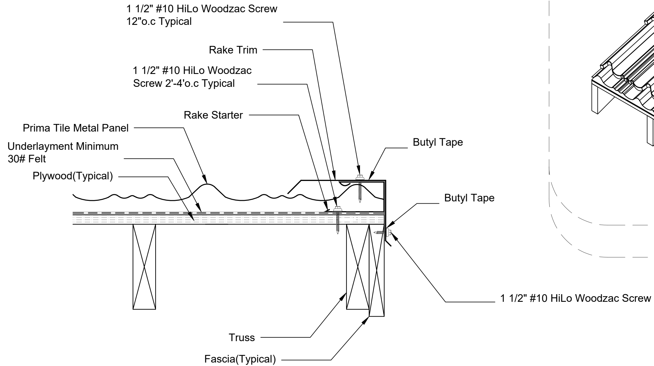
Rake Trim W/ Starter Section Scale 3"=1'
