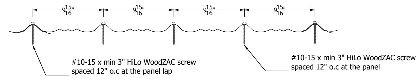
Fastening Pattern For HVHZ Construction
