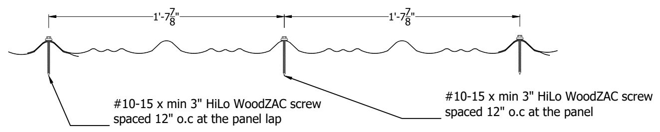
Fastening Pattern For Non-HVHZ Construction
