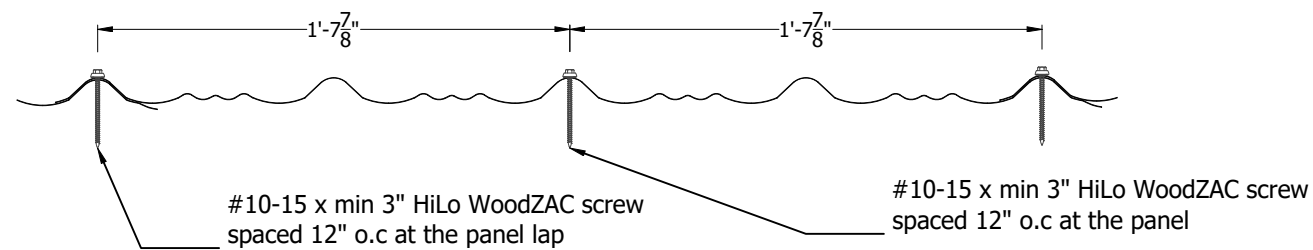
Fastening Pattern For Non-HVHZ Construction
