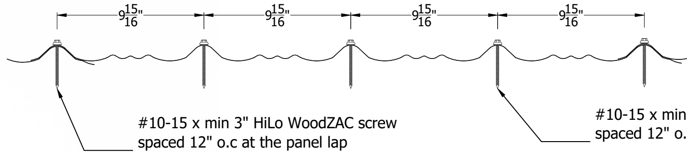
Fastening Pattern For HVHZ Construction
