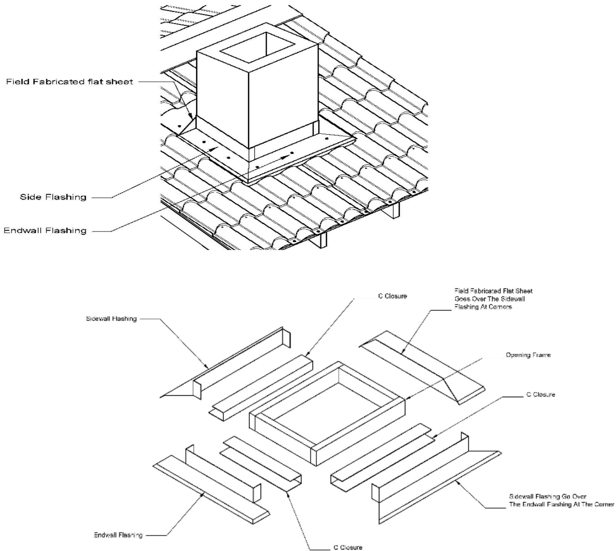
Roof Opening Flashing Detail
