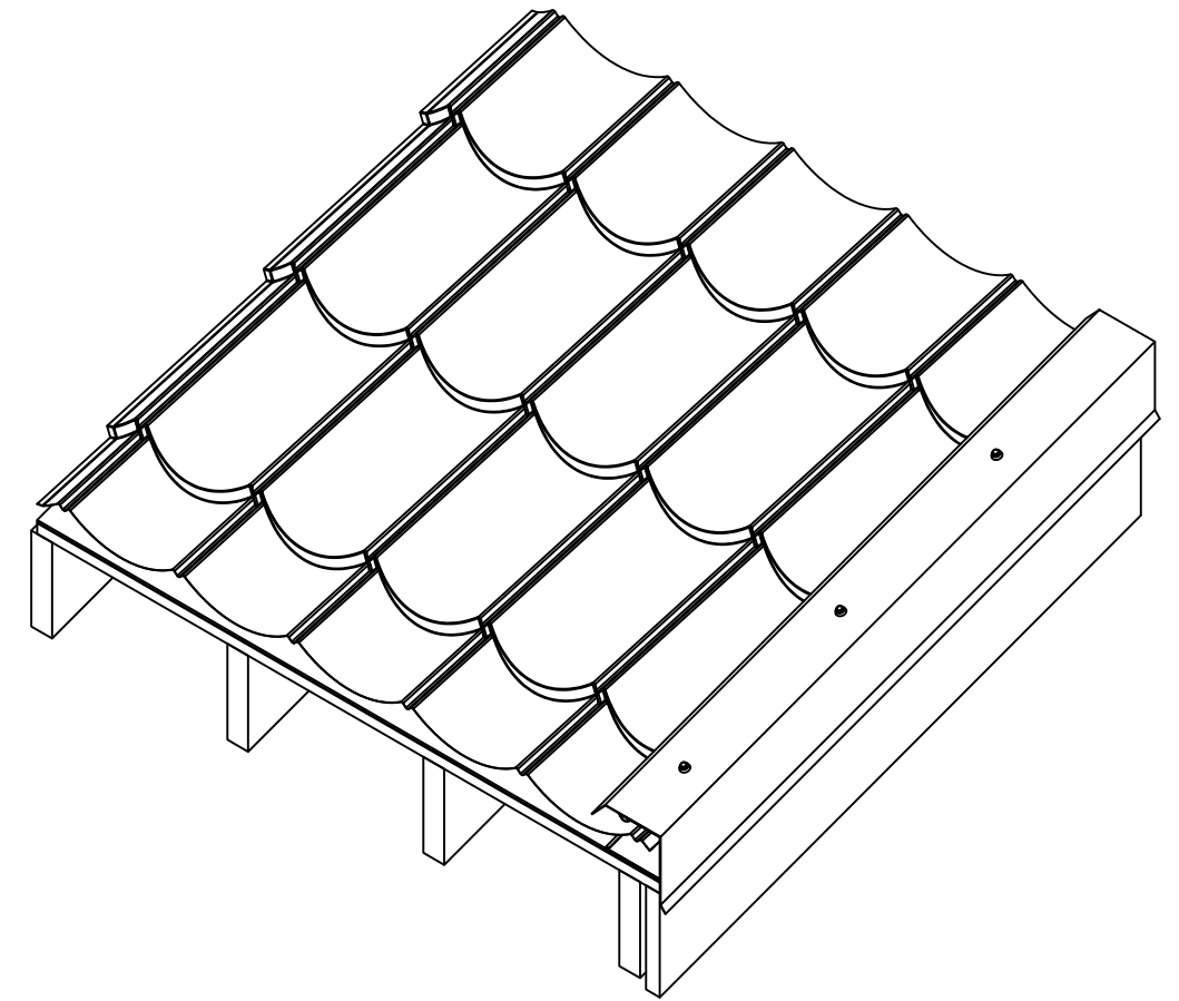
Isometric View
