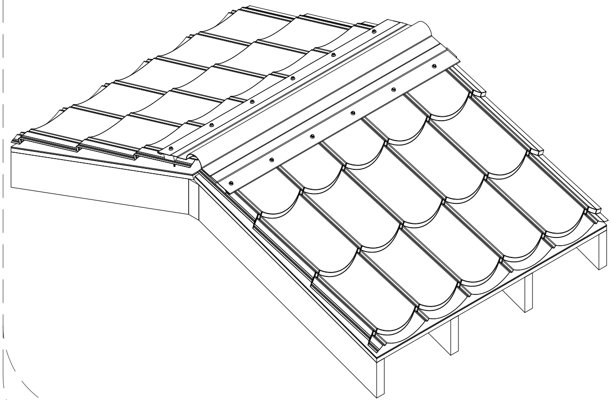
Isometric View
