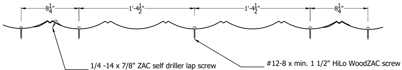
Fastening Pattern For Non-HVHZ Construction
