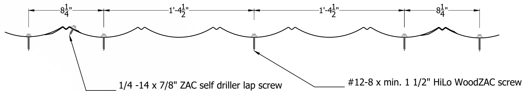
Fastening Pattern For Non-HVHZ Construction
