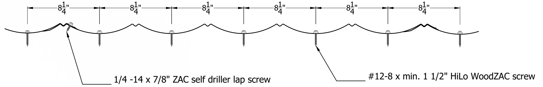
Fastening Pattern For HVHZ Construction
