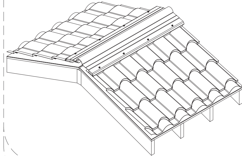
Isometric View
