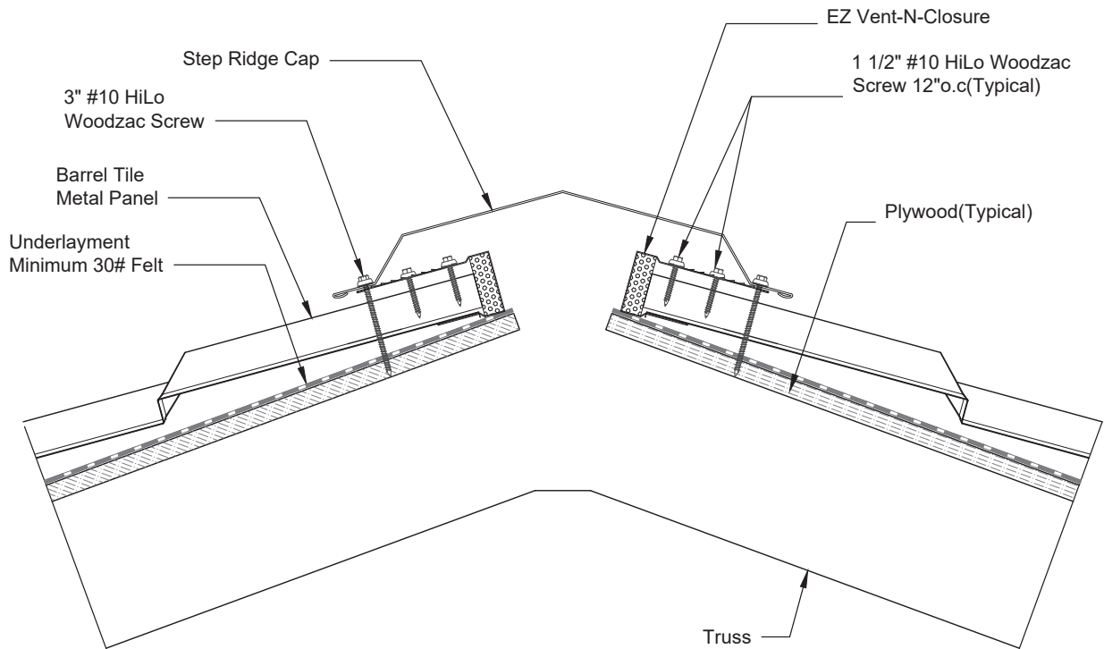
Roof Ridge Section Scale 3"=1'
