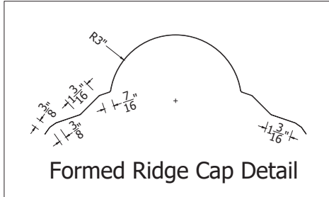
Roof Ridge Section Scale 3"=1'
