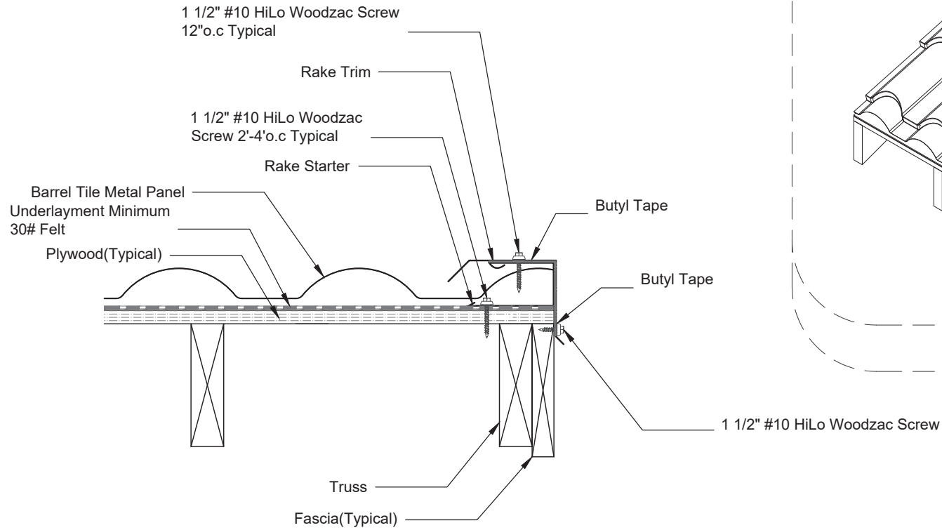
Rake Trim W/ Starter Section Scale 3"=1'
