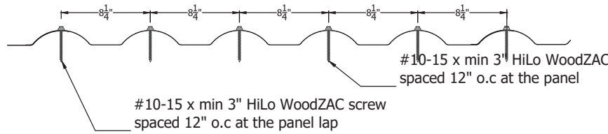
Fastening Pattern For HVHZ Construction
