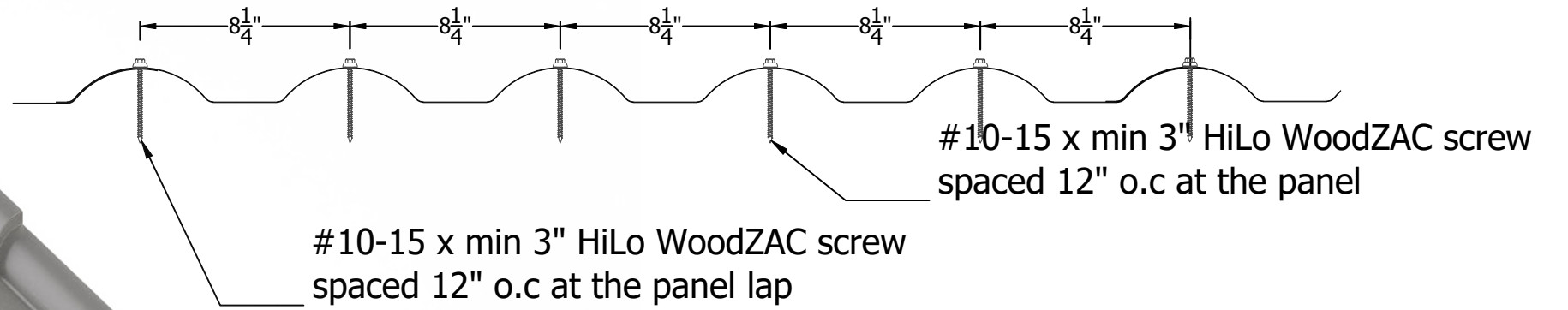
Fastening Pattern For HVHZ Construction
