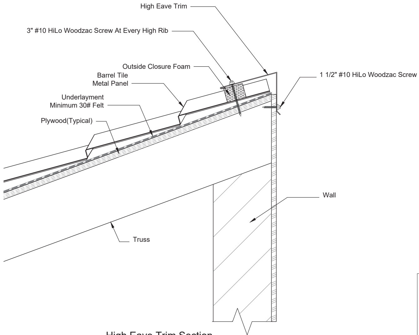
High Eave Trim Section Scale 3"=1'
