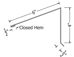
High Eave Trim Detail
