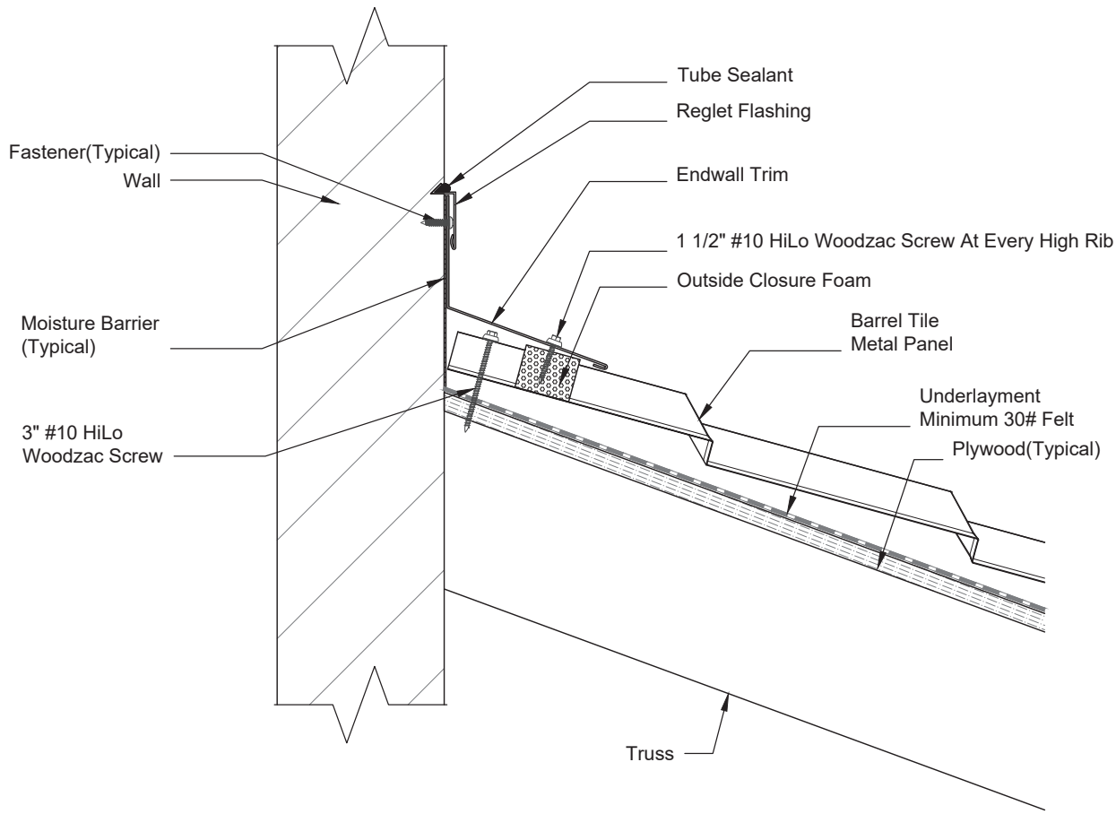
Reglet Flashing Detail Scale 3"=1'
