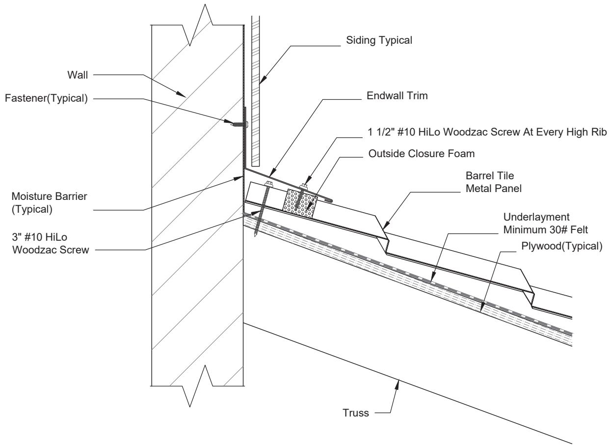
End Wall Section Scale 3" = 1'
